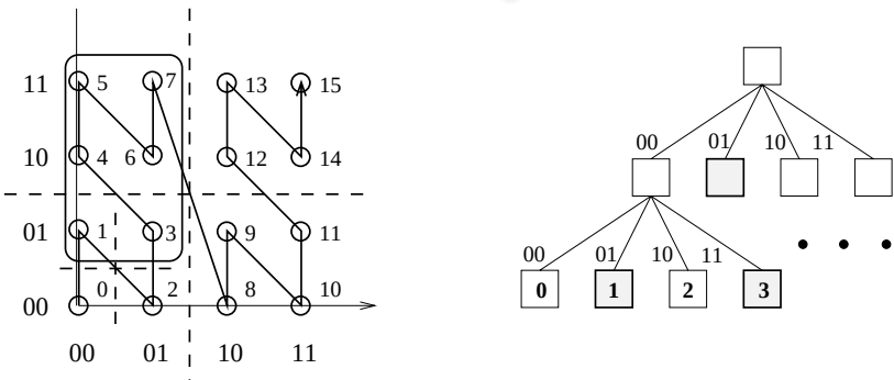
Figure 26.3 Z-Ordering and Region Quad Trees
