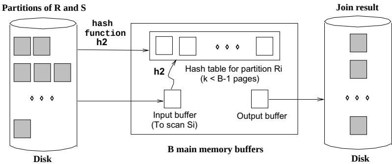
Figure 12.11 Probing Phase of Hash Join
