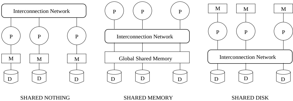
Figure 21.1 Physical Architectures for Parallel Database Systems
